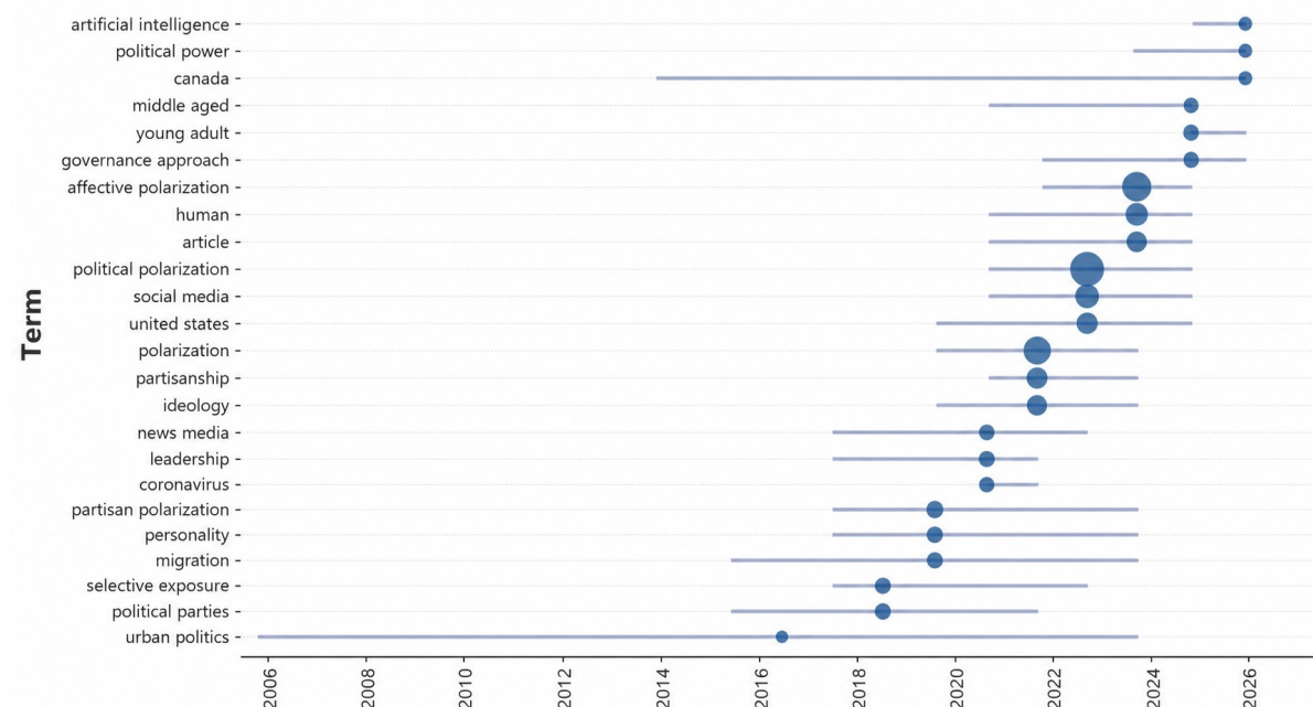
Figure 1. Trend Topics in Political Polarization Research (1974–2026)
