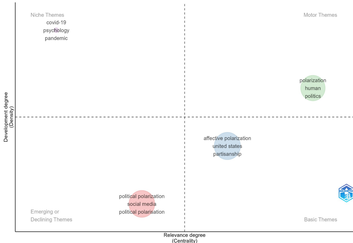
Figure 2. Thematic Map of Political Polarization Research Based on Keyword Co-occurrence
